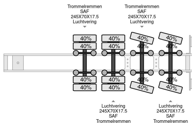
Faymonville F-S44-1AAA 4 AXLE, 2 STEERING AXLE, 7.9 M...
