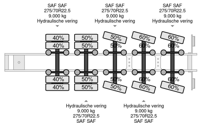
Nootboom OVB-90-05 - 5 AXLE SAF + 3 AXLE STEERING
