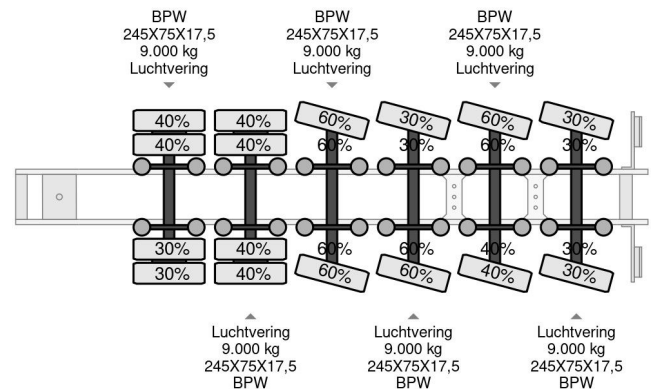
ES-GE 6 SOU-4H-1N, 6 AXLE, 4 AXLE STEERING, 2 LIFT, 8...
