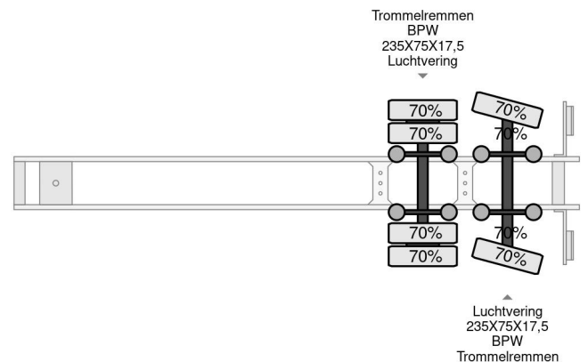
Broshuis 21N58A, 2 AXLE LAST AXLE STEERING, EXTEND...
