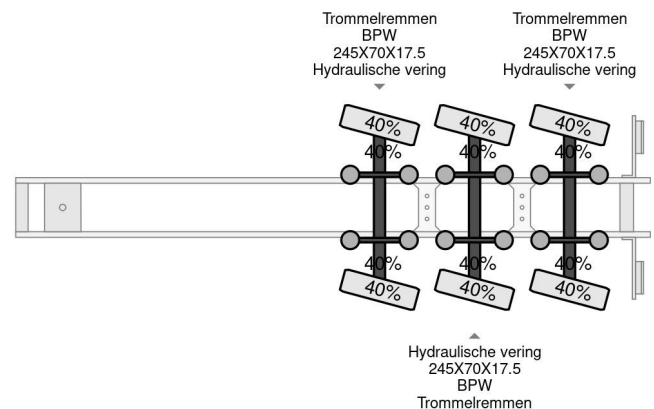
Nooteboom EURO 54-03 3 AXLE STEERING, EXTENDABLE
