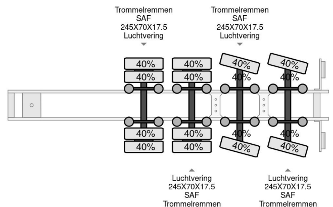
Faymonville F-S44-1AAA 4 AXLE, 2 STEERING AXLE, 7.9 M...
